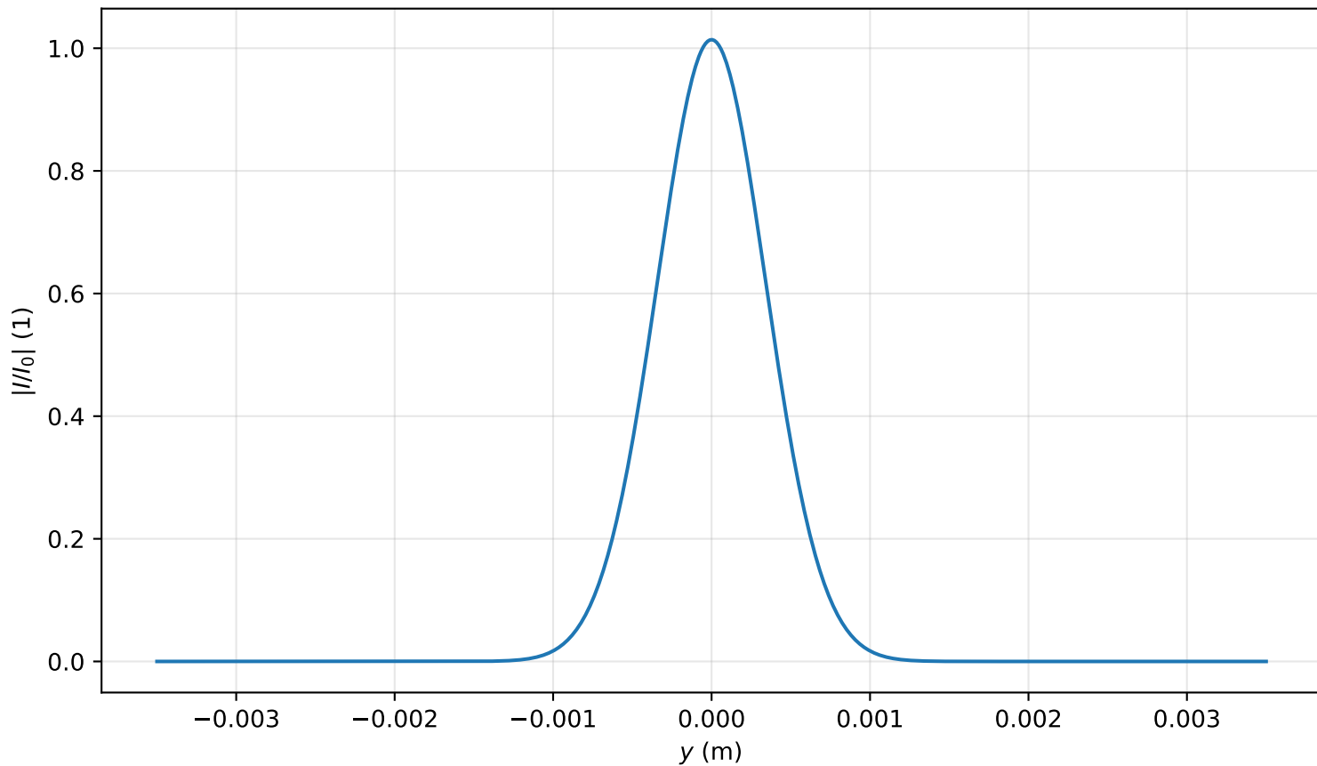
Intensity profile I(x=0, y, z=0.159)/I_0 , P_{in}=0.8P_{cr} , artificial time
